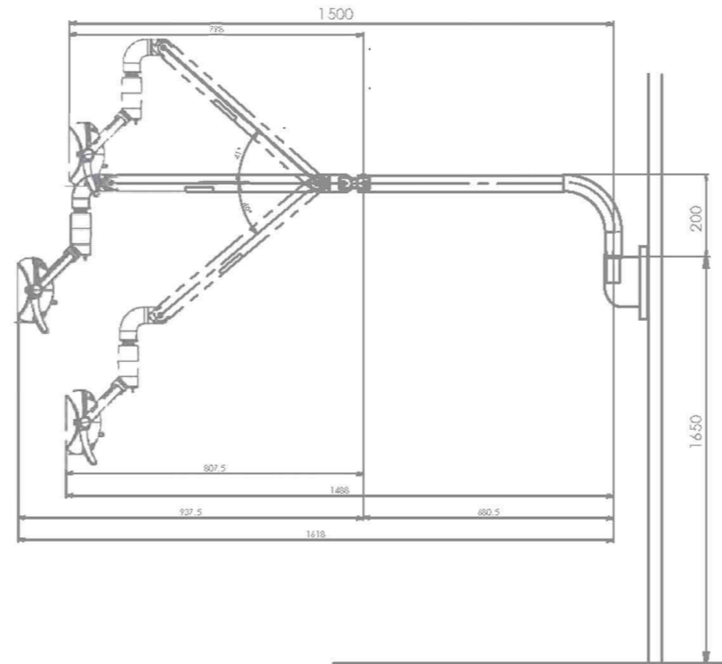
Polaris – Wandmontage
